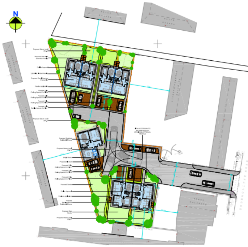
PROPOSED SITE PLAN Scale: 1:1000
